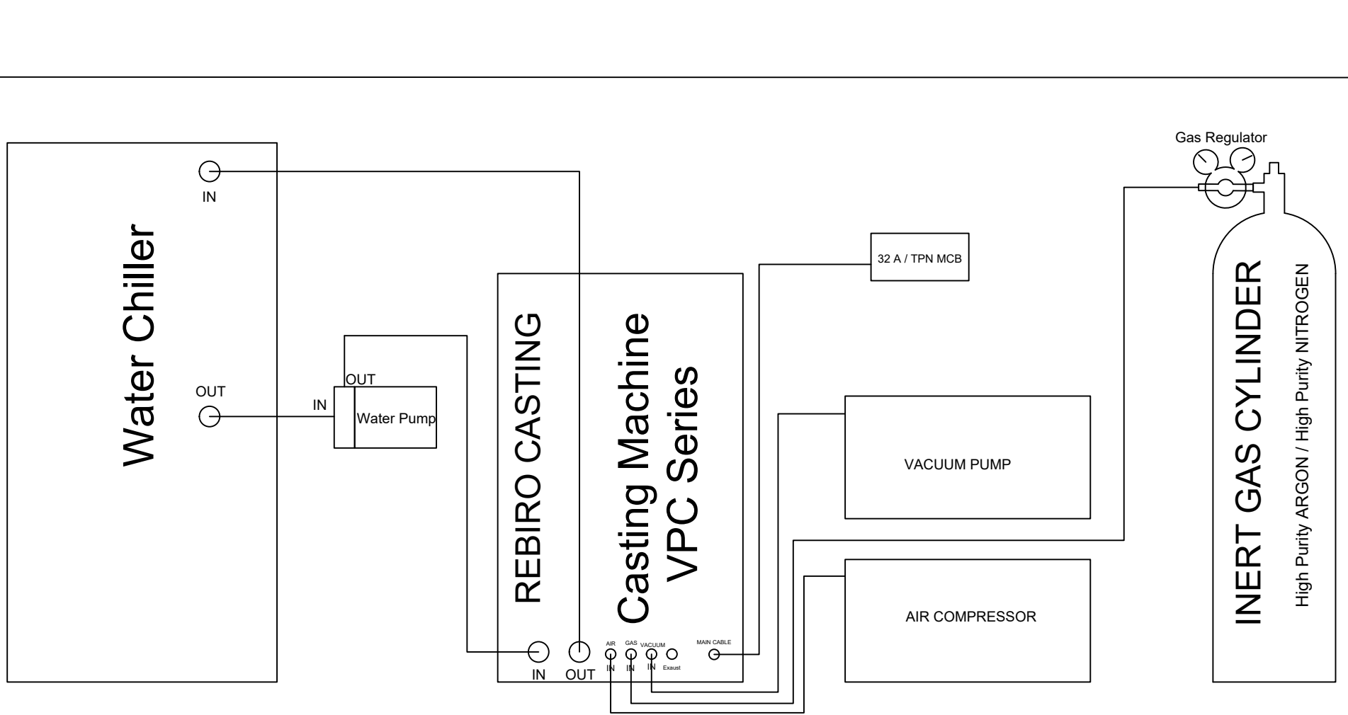
Schematic Block Diagram of SINGLE Water Pump.
